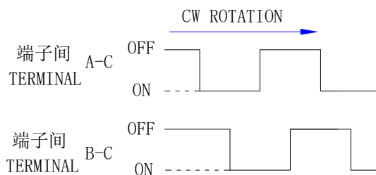
输出信号波形图 OUTPUT SIGNAL WAVEFORM FIGURE
